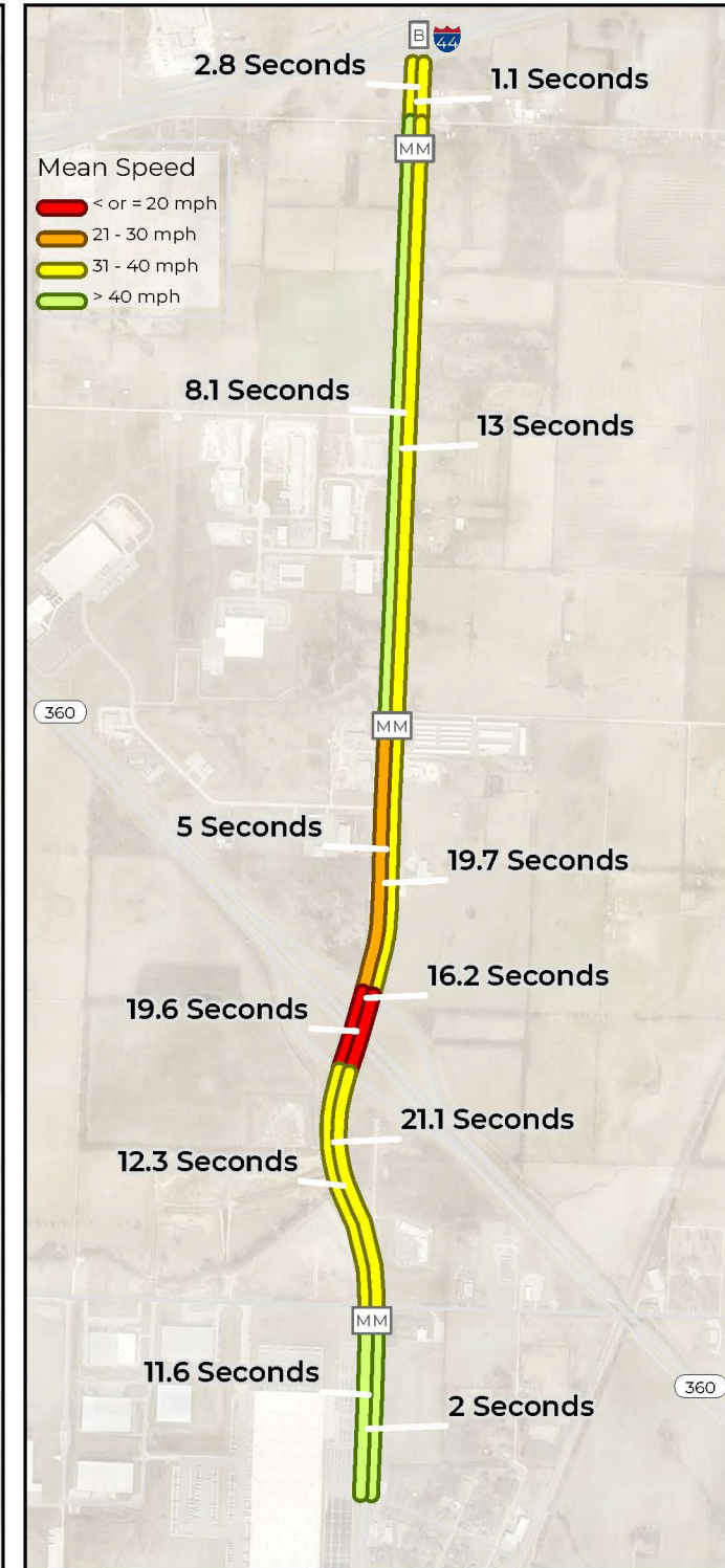
2050 Project Build (LRTP) Mean Delay
