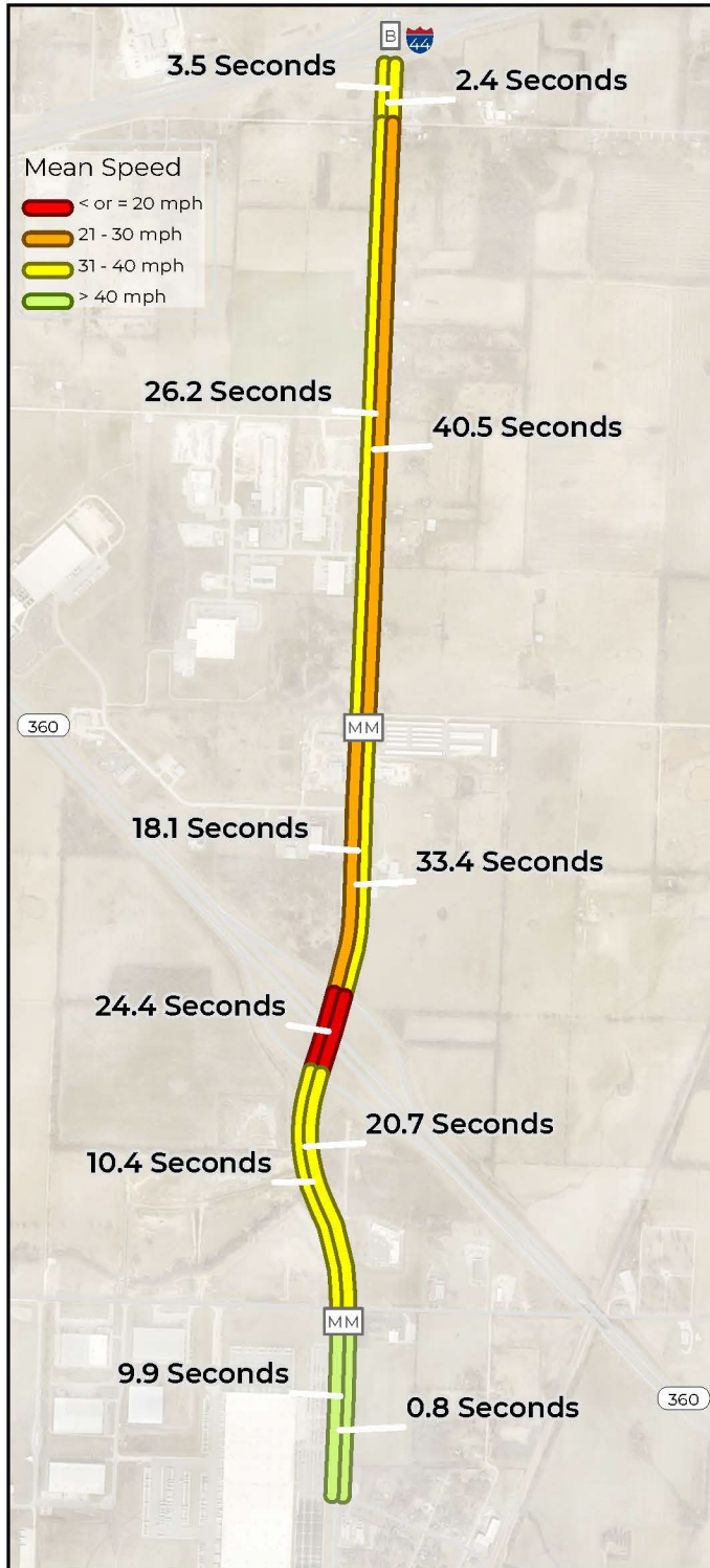
2024 Existing & Committed Mean Delay
